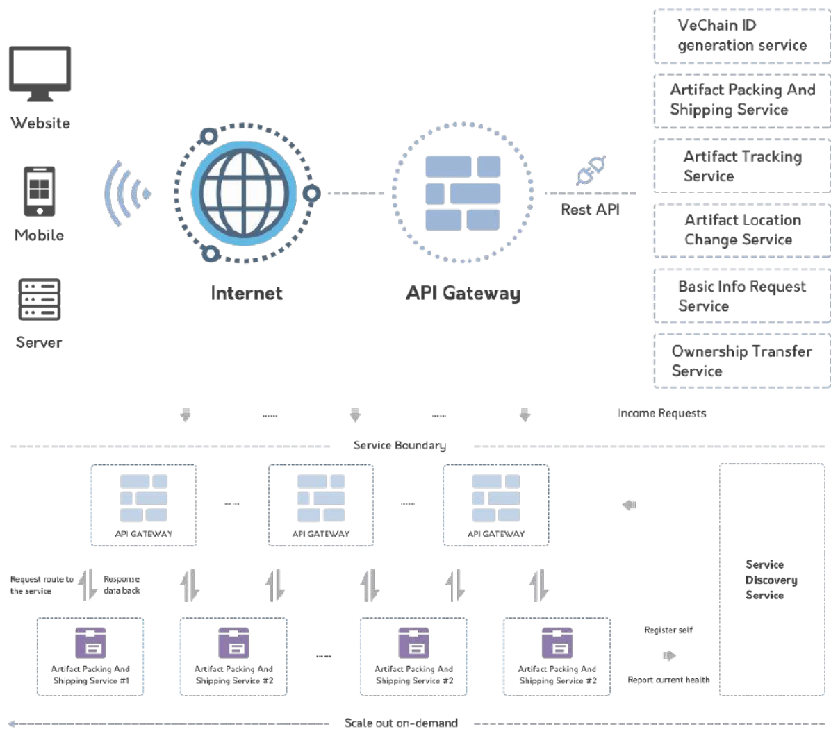
Figure 5.3.5.1 API Gateway-1
