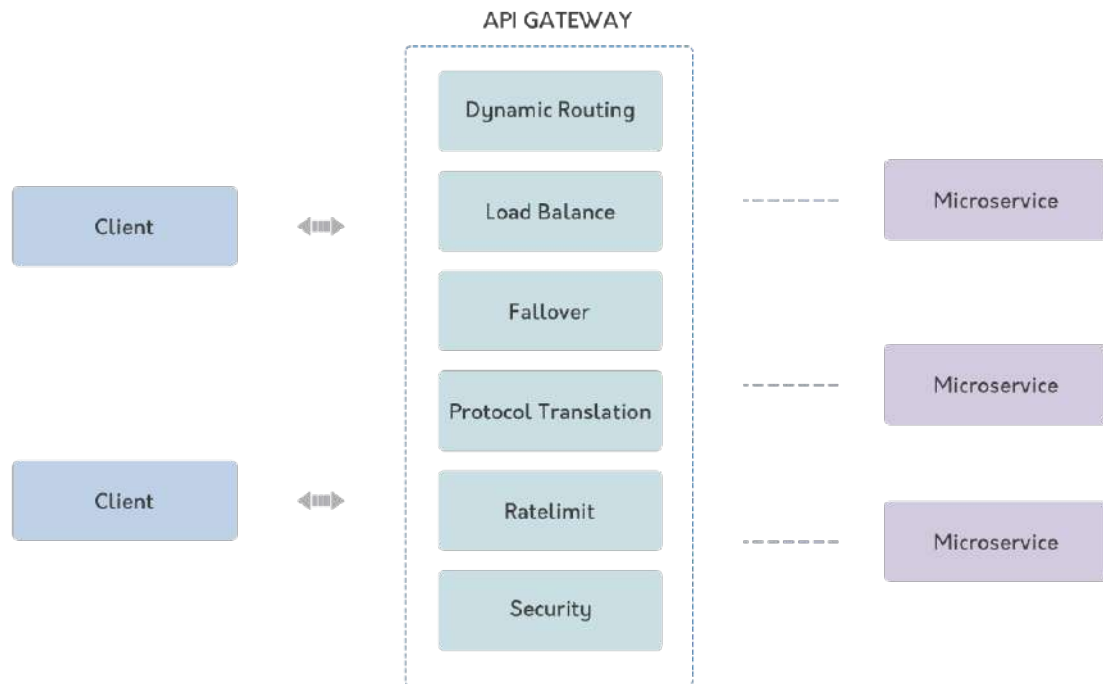
Figure 5.3.5.2 API Gateway
